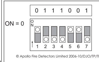
Fig 2. Example of Address 78
