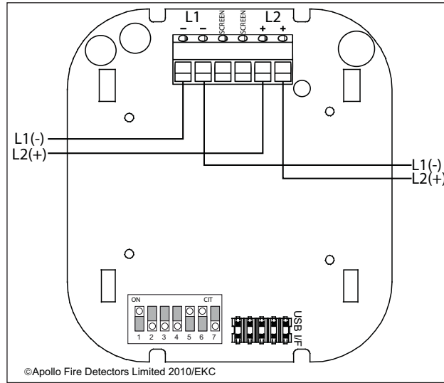
Fig 1. PCB outline
