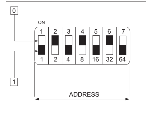
Fig 3. DIL Switch
