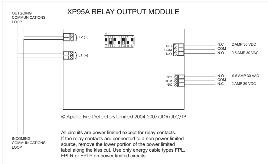
Fig 2. Wiring Diagram for XP95A Relay Output Module
